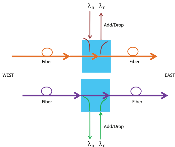
Schematic representation of Plexstar OADM
